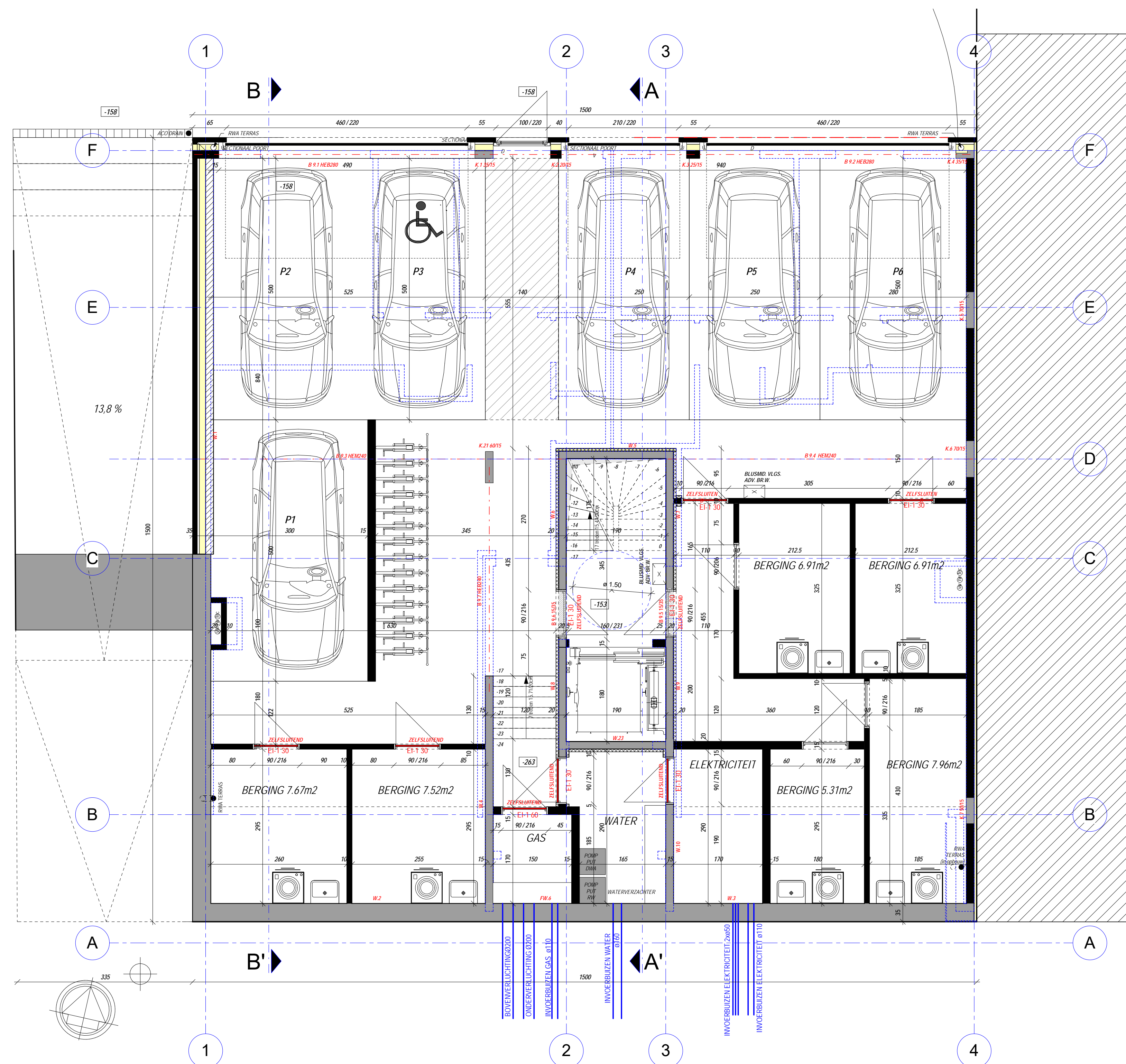
KELDERPLAN
